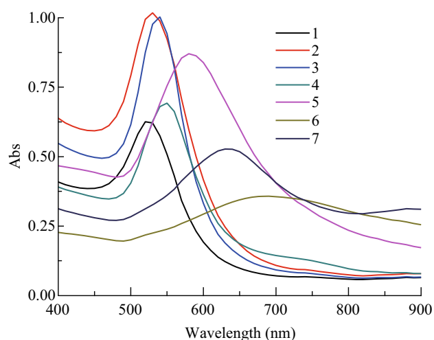
Fig. 3 UV-Vis spectra of gold nanoparticles: (1) GNSs 20.0 \pm 1 nm, (2) GNSs 35.1 \pm 2.3 nm, (3) GNSs 50.4 \pm 1.6 nm, (4) GNSs 70.2 \pm 1.8 nm, (5) GNSs 100.2 \pm 2.0 nm, (6) GNPNs 100.1 \pm 5.7 nm and (7) GNSTs 64.3 \pm 3.0 nm
