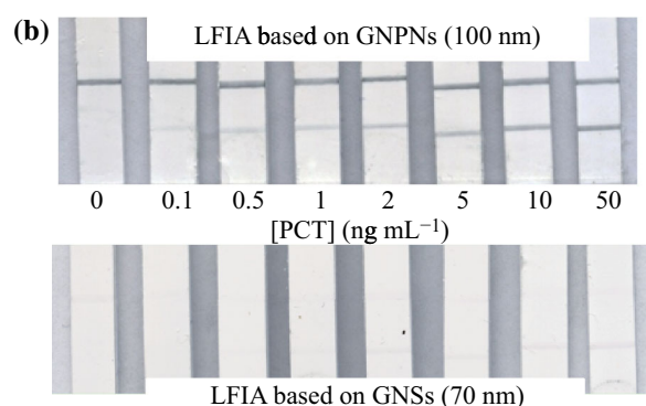
Fig. 5 a Calibration curves of LFIA for PCT detection based on GNSs, GNPNs, and GNSTs. b Color intensity in the analytical zone for GNPN-based and GNS-based LFIA (70 nm)
