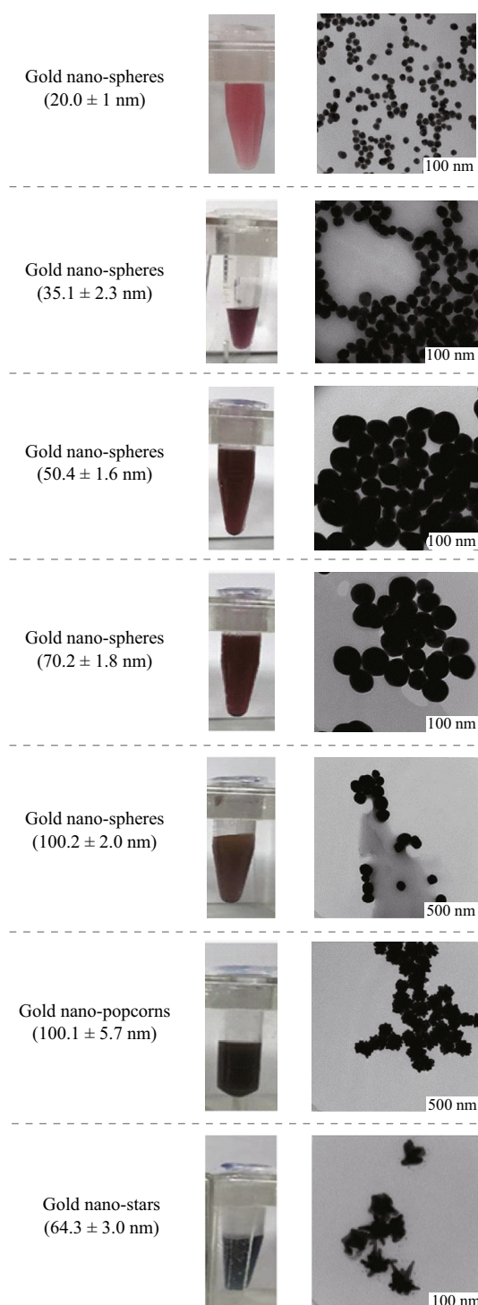
Fig. 2 Characterization of GNSs, GNPNs, and GNSTs: photograph of colloidal solutions and TEM images of gold nanoparticles
