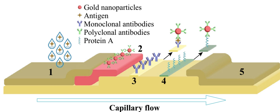
Fig. 1 Scheme of LFIA using gold nanoparticles as labels: (1) Sample pad, (2) Conjugate pad, (3) Test line, (4) Control line, (5) Absorbent pad
