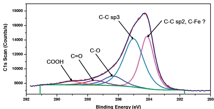
Fig. 4 High resolution XPS C 1s carbon peak observed for the \text{Fe}_7\text{C}_3@C sample.
