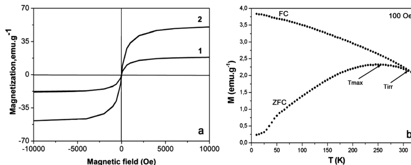
Fig. 5 The curves of magnetization versus the applied field obtained at room temperature for the as-prepared sample (1) and separated fraction of \text{Fe}_7\text{C}_3@C NPs (2) (a). The curves of zero field and field cooled magnetization ( M_{\text{ZFC}} and M_{\text{FC}} ) versus temperature (from 5 to 325 K) (b).
