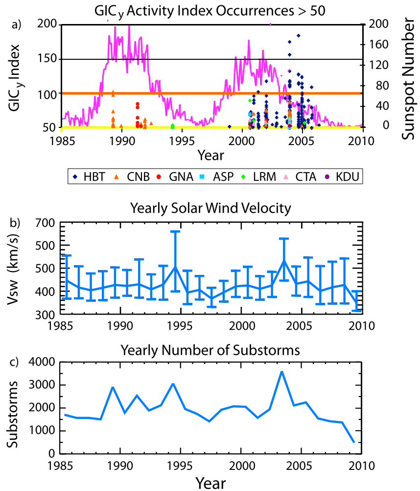
Figure 10. (a) Adapted version of Figure 7 of Marshall et al. (2011), showing GICy indices >50 from magnetometer locations across Australia (colored dots, corresponding to the vertical scale on the left side) and the solar sunspot number (pink trace, corresponding to the vertical scale on the right), from 1985 through 2009. The horizontal yellow and orange lines are the lower limit thresholds for the “low” and “moderate” threat levels defined in that study. (b) Yearly medians and 25th and 75th percentile values (lower and upper bars) of the solar wind velocity and (c) Yearly numbers of substorm onsets from the Newell and Gjerloev (2011) list on SuperMAG, respectively, from 1985 through 2009.
