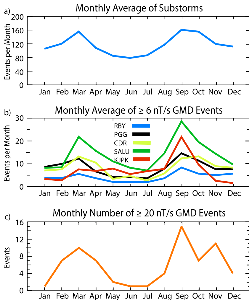
Figure 7. Monthly distributions of substorms and GMDs. Panel a shows the average number of events per month from 2011 through 2021 (no year 2022 substorm list was available on SuperMAG as of 10/11/2023). Panel b shows the weighted monthly average number of \geq 6 nT/s GMDs from 2011 through 2021, and panel c shows the distribution of >20 nT/s GMDs from 2011 through 2022.
