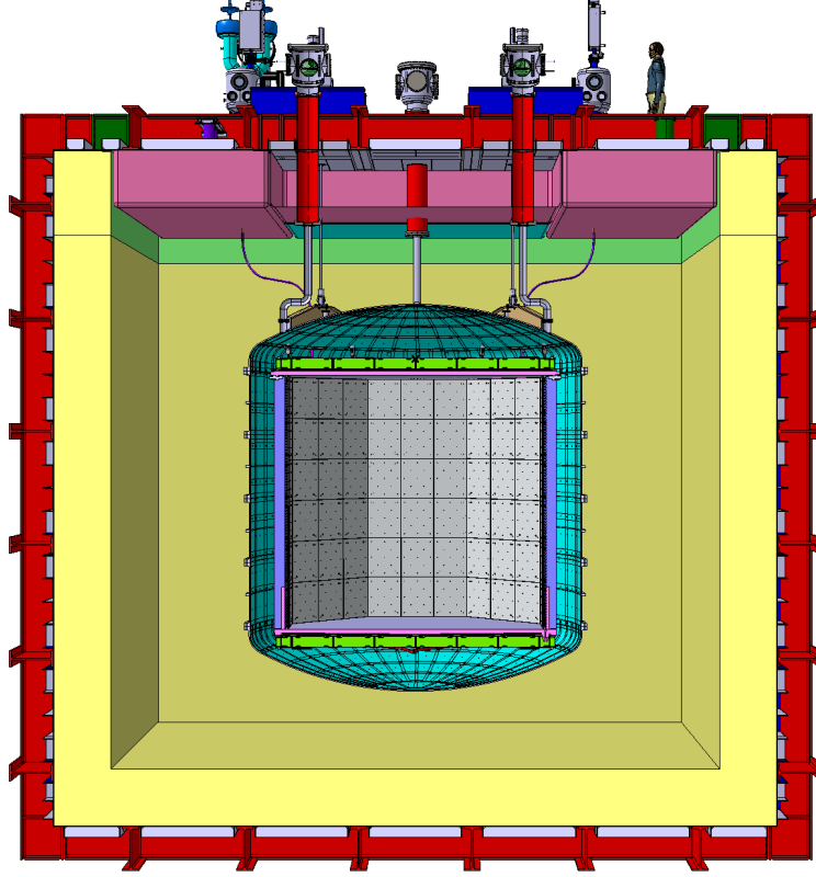
Figure 1. The picture shows a drawing of the DarkSide-20k apparatus. The innermost part is the TPC: the position of the Gd-PMMA lateral walls (which form an octagon) is shown in violet, while the pure PMMA windows at the top and bottom are depicted in pink. Above and below the pure PMMA windows there are the Gd-PMMA endcaps, which are represented in bright green. The TPC and Veto are contained in a stainless steel vessel, light blue in the picture, that holds the underground liquid argon. The vessel is hanging from the top of a big membrane cryostat (in red and yellow), that will be filled with atmospheric liquid argon. Neutrons moderated and captured in the Gd-PMMA (violet and green), produce \gamma rays that induce scintillation in the surrounding liquid argon, therefore they are tagged.
