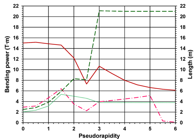
Fig. 6 Magnetic flux density bending component integrals (left scale, solid and dash-dotted lines), and the length of the charged particle trajectory (right scale, dashed and small dotted lines) in the inner tracker (smooth and dashed lines) and in the muon system (dash-dotted and small dotted lines) vs. the pseudorapidity
