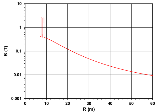
Fig. 5 Magnetic flux density out of the coil in the coil central plane vs. radius. The two peaks at about 2.5 T correspond to two barrel layers of the magnet flux return yoke
