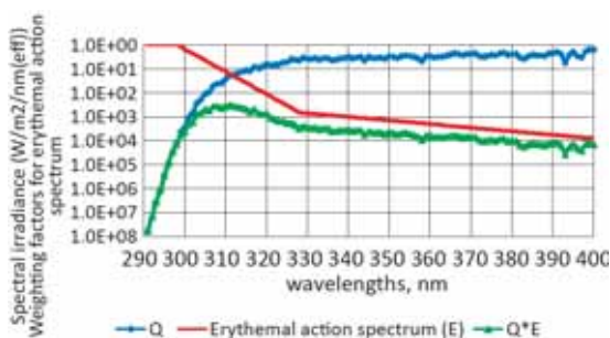
Fig. 1. Spectral distribution of UV radiation ( Wm\text{-}2nm ) ( Q ), erythral action spectrum ( E ), and UV radiation weighted on erythral action spectrum ( Q_{er} ) ( Wm\text{-}2nm_{eff} ). Model calculation (solar zenith angle 60 degree, total ozone content = 300 DU), clear sky.
