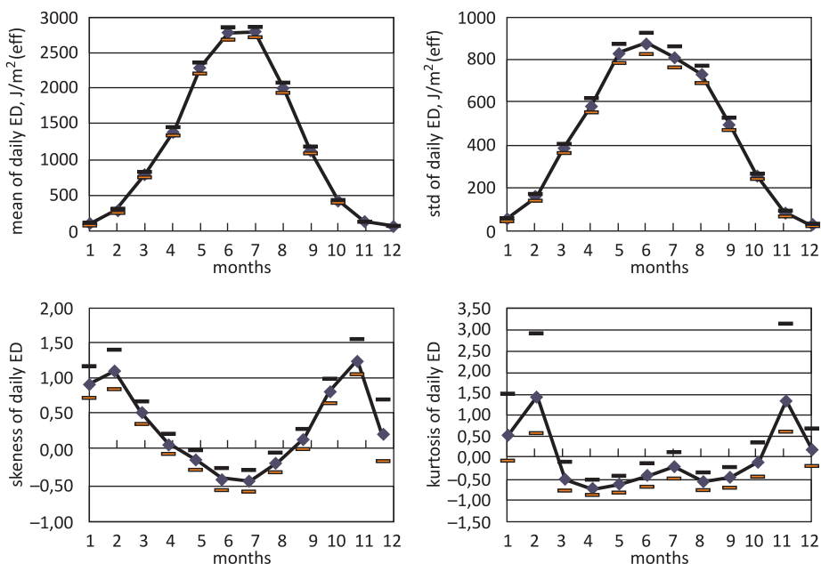
Fig. 4. Seasonal changes in ED daily mean, standard deviation, skewness, and kurtosis at a 95% significance level.
