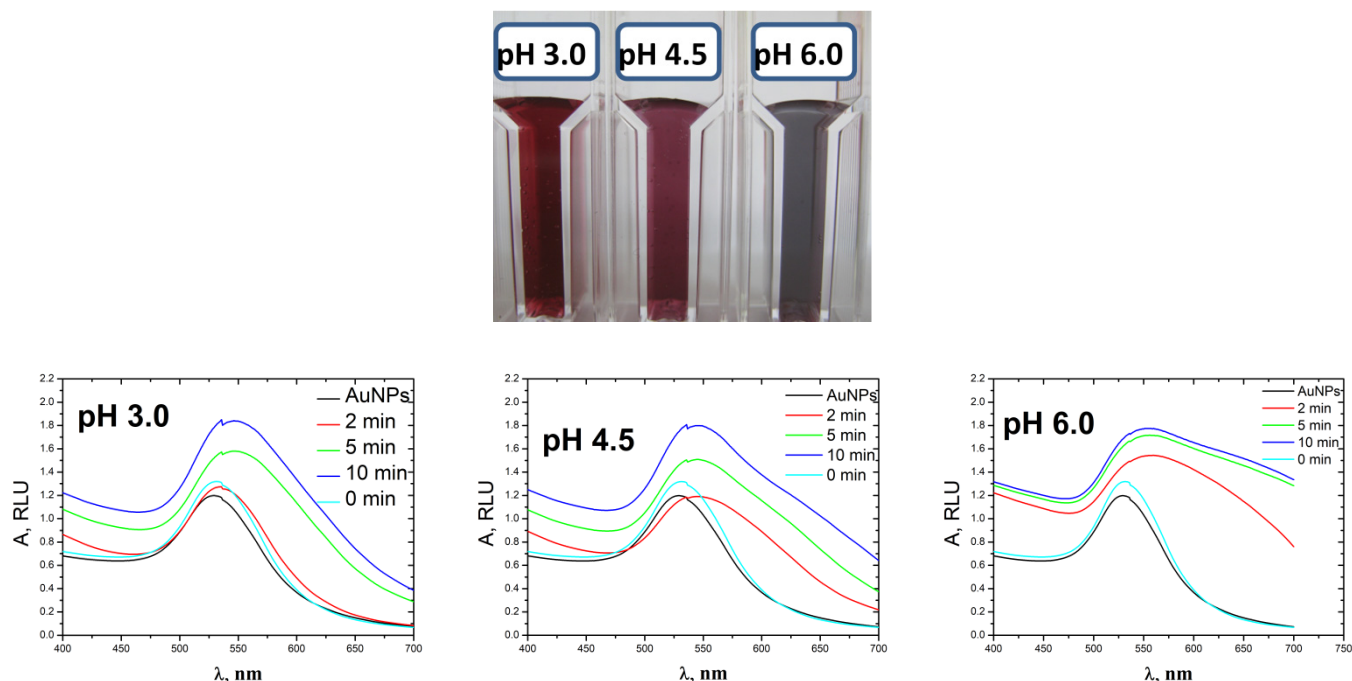
Figure 3. Spectra of streptavidin-AuNP conjugate during the reduction of \text{HAuCl}_4 with \text{NH}_2\text{OH} at different pH and reaction time. The black lines correspond to the spectra of colloidal solutions without amplification.
