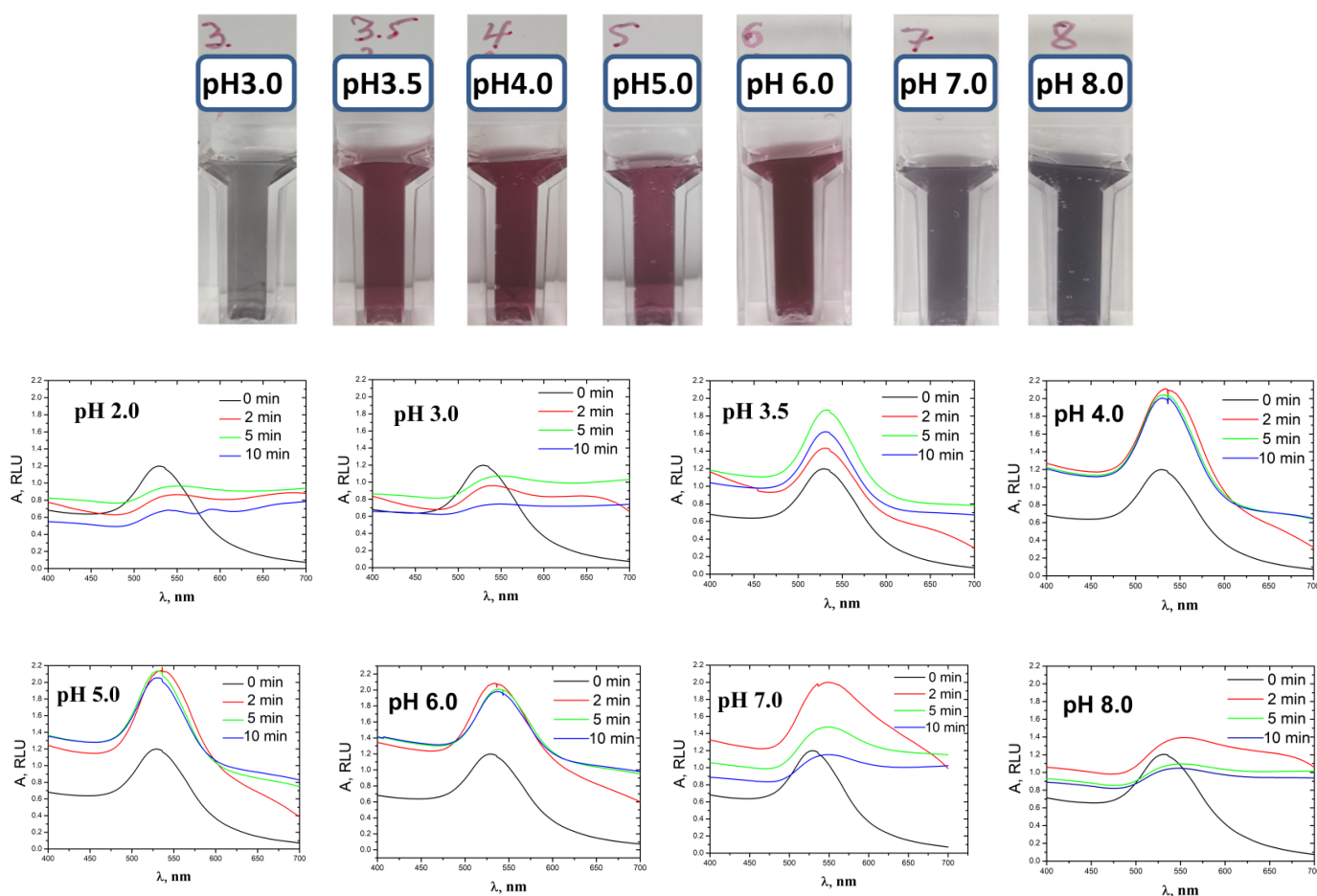
Figure 2. Spectra of colloidal suspensions of gold nanoparticles during the reduction of HAuCl_4 with NH_2OH at different pH and reaction time. The black lines correspond to the spectra of the colloidal suspensions without amplification.
