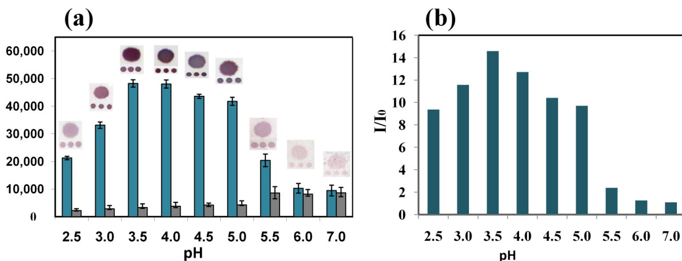
Figure 4. Absolute intensities of staining of specific spots (blue) and areas around the spots (gray) after AuNP enhancement at different pH values (a); signal-to-noise ratios at different pH values (b). Hybridization of 150 pM of target oligonucleotide.
