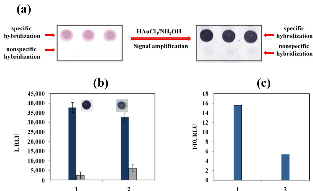
Figure 8. Images of nitrocellulose microarrays before and after the enhancement of AuNP labels using an enhancement solution at optimized reagent concentrations and pH (0.7 mM tetrachloroauric acid and 50 mM hydroxylamine, pH 3.5) (a); the staining intensities of specific (blue) and background (gray) spots with different orders of reagent mixing (b); and signal-to-noise ratios with different orders of reagent mixing (c). Target oligonucleotide (50 pM) was hybridized on the microarrays. 1—the pH value of tetrachloroauric acid solution was adjusted to 3.5 before the mixing with hydroxylamine; 2—the reagents were mixed without adjusting the pH value.
