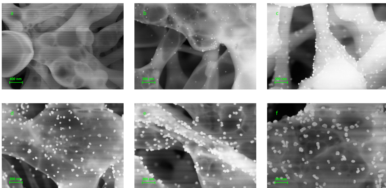
Figure 5. SEM images of the specific and control spots after hybridization of the membrane microarray with 150 pM of target oligonucleotide followed by enhancement procedure at pH range from 2.5 to 4.5. (a) Control spot; (b) specific spot without enhancement; (c–f) specific spot after enhancement at pH 2.5 (c); pH 3.0 (d); pH 3.5 (e); and pH 4.5 (f).
