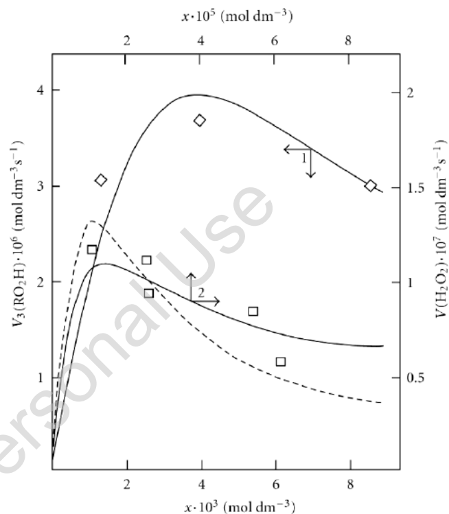
Figure 3: (1, \diamond ) Reconstruction of the functional dependence of the 2-methylbenzyl hydroperoxide formation rate V_3(RO_2H) on the dissolved oxygen concentration x from empirical data (points) using Eq. (3a) (model optimization with respect to the parameter \alpha ) for the o -xylene–oxygen system at 373 K [46] (standard deviation of S_Y = 5.37 \times 10^{-7} ). (2, \square ) Reconstruction of the functional dependence of the total hydrogen peroxide formation rate V_3, \gamma(H_2O_2) on the dissolved oxygen concentration x from empirical data (symbols) using Eqs. (3a) and (12) with \beta = 0 (model optimization with respect to the parameter \alpha ) for the \gamma -radiolysis of water saturated with hydrogen and containing different amounts of oxygen at 296 K [63] ( S_Y = 1.13 \times 10^{-8} ). The dashed curve described V_3(H_2O_2) as a function of the oxygen concentration x based on Eq. (3a) (model optimization with respect to \alpha ) and the experimental data of curve 2 ( S_Y = 1.73 \times 10^{-8} ).
