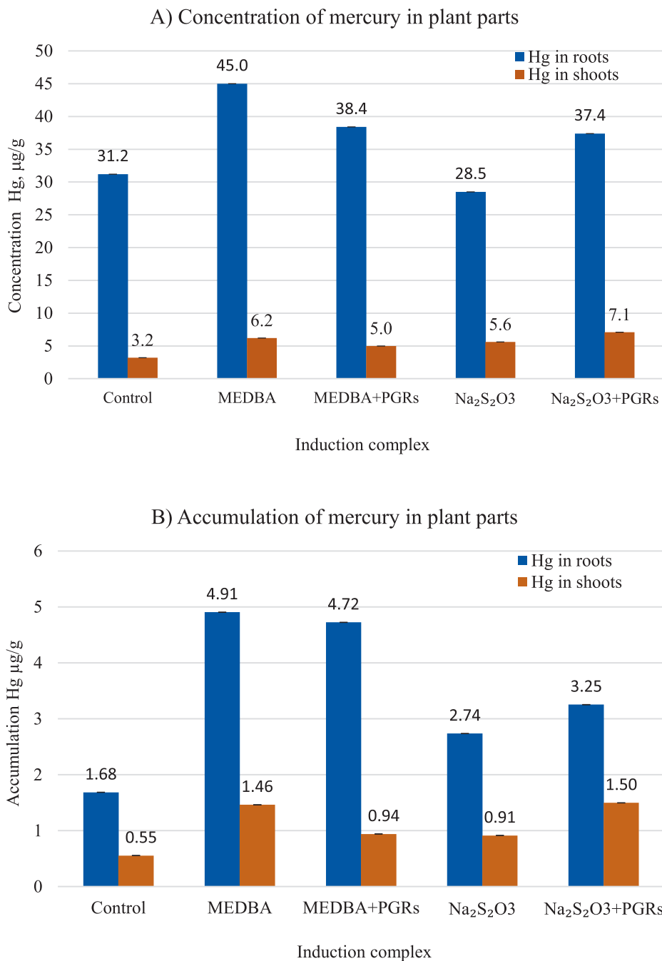
Fig. 3. Characteristics of absorption and accumulation of mercury in plant parts using various induction complexes: A) concentration of mercury in plant parts; B) accumulation of mercury in plant parts.
