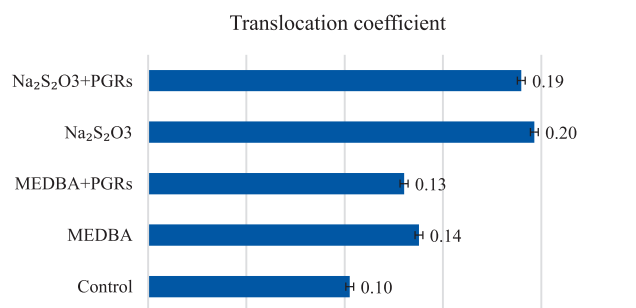
Fig. 4. Translocation coefficients of mercury when using various induction complexes in phytoextraction.
