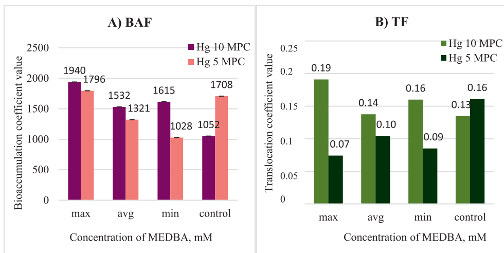
Fig. 2. Bioaccumulation (A) and translocation (B) coefficients at various MEDBA concentrations.
