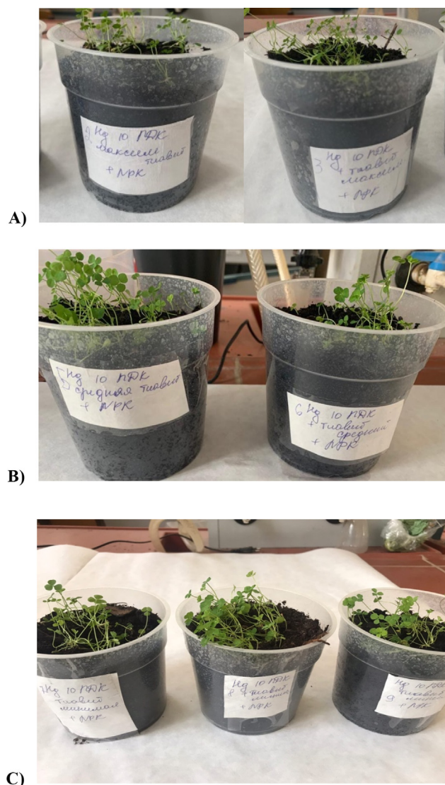
Fig. 1. Photographs of T. repens at different amounts of MEDBA introduced into the substrate with a mercury contamination level of 10 MPC: A) maximum; B) average; C) low.
