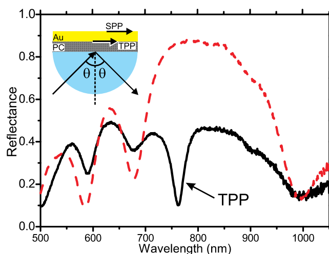
FIG. 1. Experimental reflectance spectra of photonic crystal (dashed curve) and Au/PC (solid curve) samples at \theta = 30^\circ for TM polarization. Inset: schematic of the experiment.
