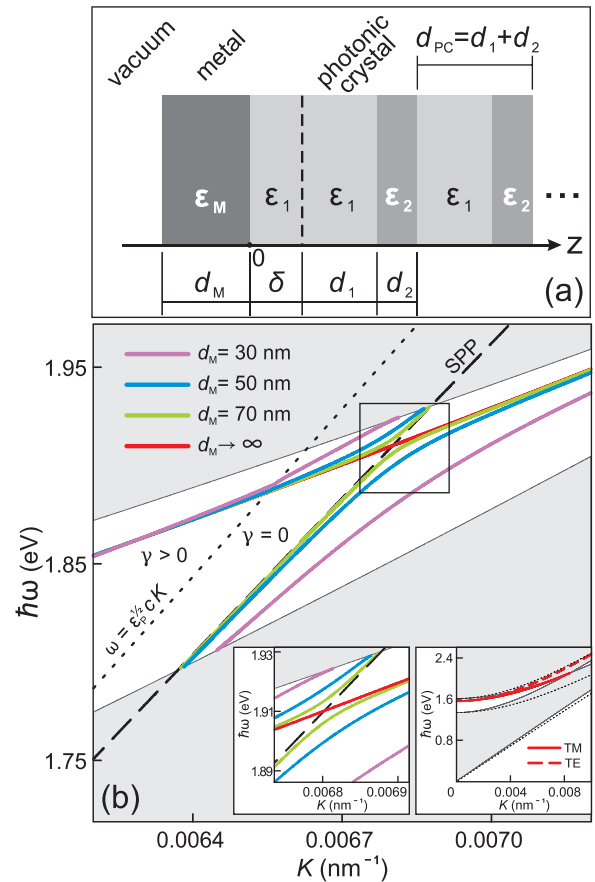
FIG. 5. (a) Model structure. (b) Dispersion of the TM TPP calculated for the model structure at specified values of d_M . Gray areas correspond to the bulk TM photonic bands of the infinite PC. Dashed line indicates the dispersion curve of the SPP at the vacuum/semi-infinite metal interface. Dotted line being the light line in the prism separates radiative ( \gamma > 0 ) and non-radiative ( \gamma = 0 ) regions. The area marked with the square is shown enlarged in the left inset. Right inset shows the dispersion curves of the TM and TE TPPs calculated for the semi-infinite metal/semi-infinite PC structure. Dotted lines represent the boundaries of the bulk TE photonic bands. The parameters used in calculations are the following: \delta = 80 nm, d_1 = 146 nm, d_2 = 109 nm, \epsilon_1 = \epsilon_p = 2.13 , \epsilon_2 = 3.80 , \epsilon_M(\omega) = 1 - (\omega_p/\omega)^2 with \hbar\omega_p = 8.87 eV.
