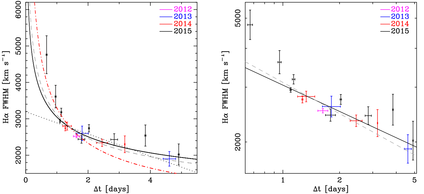
Figure 13. Evolution of the FWHM of the H \alpha emission line following the eruption of M31N 2008-12a (left: linear axes, right: logarithmic axes). See the key for data point identification. The dotted black line shows a simple linear least-squares fit to the 2012–2015 data (gradient = -300 \pm 70 \text{ km s}^{-1} \text{ day}^{-1} , \chi^2_{\text{dof}} = 3.9 ; if the first two data points are ignored \chi^2_{\text{dof}} reduces to 3.1, the gray dashed line a power-law of index -1/3 ( \chi^2_{\text{dof}} = 2.7 ; Phase II of shocked remnant development), the red dot-dashed line a power-law of index -1/2 ( \chi^2_{\text{dof}} = 5.8 ; Phase III), and the solid black line the best fit power-law with index -0.28 \pm 0.05 ( \chi^2_{\text{dof}} = 2.7 ), see text for details. These observations indicate that the ejecta shock pre-existing circumbinary material close to the central system. The most likely conclusion is that the donor is seeding the local environment via a stellar (red giant) wind.
