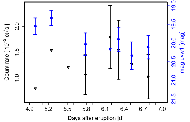
Figure 6. Swift XRT count rates (black) and UVOT uvw1 magnitudes (blue) used for estimating the SSS turn-on time as day 5.6 \pm 0.7 after eruption (cf. Figures 3 and 4.)
