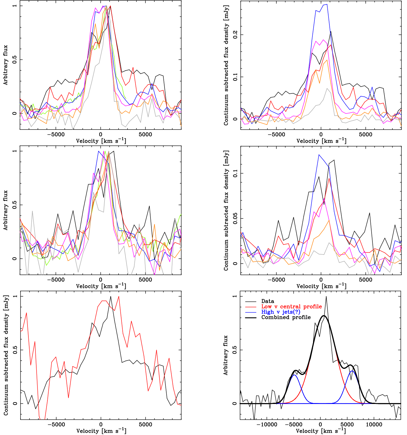
Figure 11. Evolution of the H \alpha ( top ) and H \beta ( middle ) line profiles following the 2015 eruption of M31N 2008-12a. Left: The peak flux of each H \alpha /H \beta line has been normalized to 1 – to indicate the evolution of the line morphology. Right: Flux calibrated spectra are shown to illustrate the change in flux of the H \alpha /H \beta emission. Bottom left: Comparison between the H \alpha and He I (5876 Å) lines at \Delta t = 0.67 days; the line blueward of the He I line ( \sim -8000 km s ^{-1} ) is N II (5679 Å). Bottom right: H \alpha line profile at t = 0.67 d, the red and the blue lines show a best-fit model of three Gaussian profiles, the thick black line their combined flux (see Section 7.4). Line colors as Figure 10 with the additional green data \Delta t = 1.10 \pm 0.01 days (KPNO; rebinned). The peak redward of H \alpha ( \sim +5300 km s ^{-1} ) is He I (6678 Å). The data in all these plots have been continuum subtracted as described in the text.
