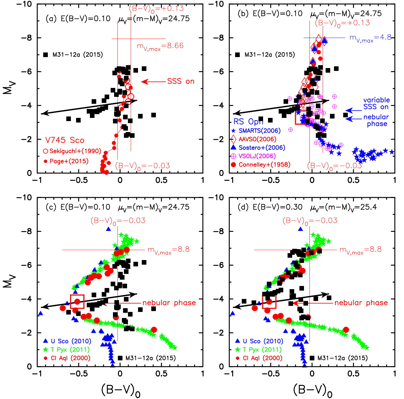
Figure 7. Color-magnitude diagrams of M31N 2008-12a for various extinctions and apparent distance moduli (indicated at the top of each plot) are compared with those of Galactic RNe. Throughout, the filled black squares denote the color-magnitude points of M31N 2008-12a from the 2013, 2014, and 2015 eruptions. In each plot the evolution of M31N 2008-12a is compared directly to (a) V745 Sco (RG-nova), (b) RS Oph (RG-nova), (c-d) U Sco and CI Aql (SG-novae), and T Pyx (MS-nova); see the plot keys and text for further details. In plot (d) the extinction toward M31N 2008-12a was allowed to vary for illustrative purposes. Given the known extinction, the track of M31N 2008-12a is closer to those of the RG-novae (a-b) than the other RNe (c-d), consistent with the interpretation that the companion is a red giant.
