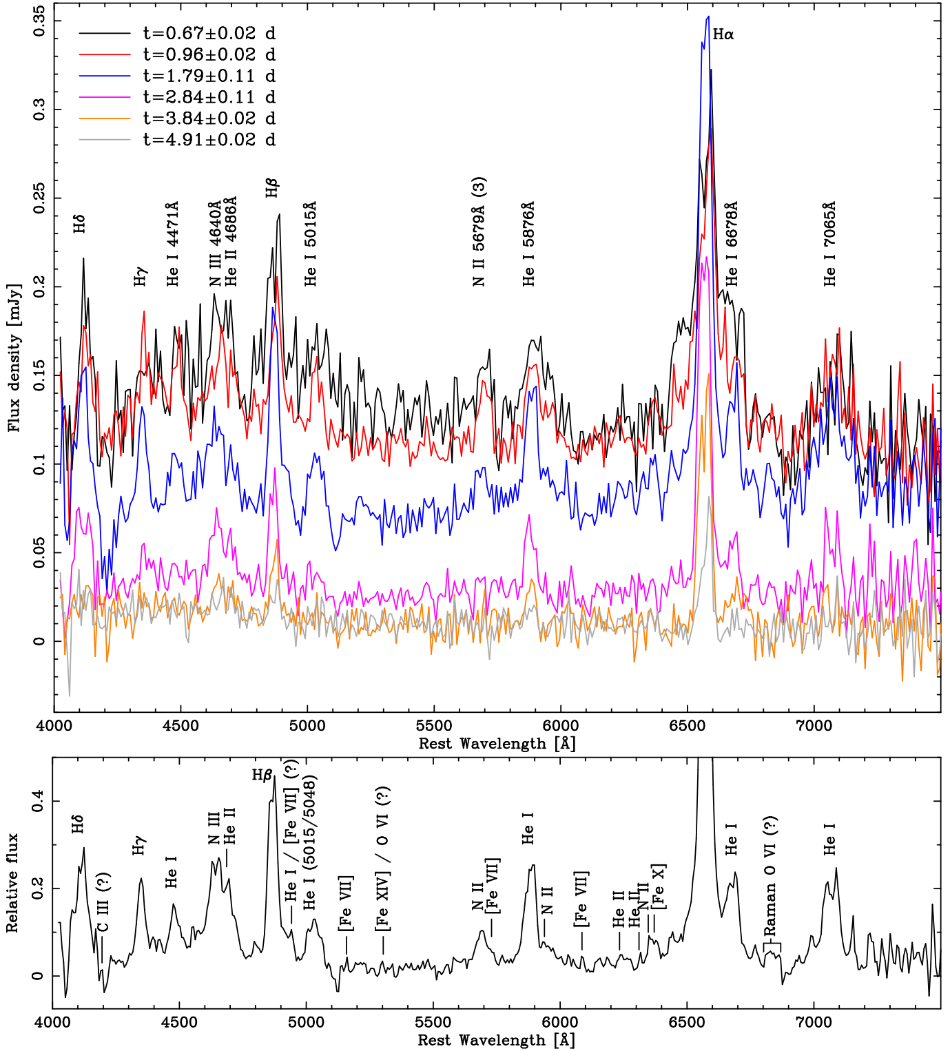
Figure 10. Top: Liverpool Telescope SPRAT flux calibrated spectra of the 2015 eruption of M31N 2008-12a, see the key for line identifiers. Spectra are consistent with the He/N canonical class of nova. Bottom: Combined spectra from the 2012, 2014, and 2015 eruptions; see text for details. Additional features, not identifiable in the individual spectra are indicated. These include tentative detections of the coronal [Fe VII], [Fe X], and [Fe XIV] emission lines, typically associated with shocks between the ejecta and surrounding material, and possibly the Raman scattered O VI emission band, a signature of symbiotic stars.
