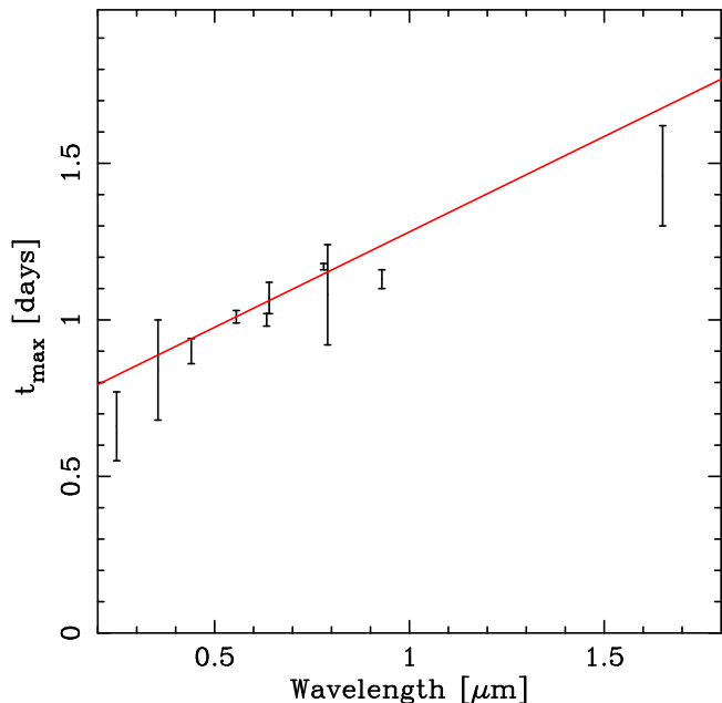
Figure 5. Evolution of the time of maximum light with wavelength. These data are consistent with the time of maximum increasing linearly with wavelength with a gradient of 0.61 \pm 0.11 days \mu\text{m}^{-1} (indicated by the red line).
