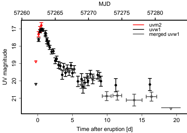
Figure 3. Unprecedentedly detailed Swift UVOT light curve for the 2015 eruption of M31N 2008-12a, showing for the first time the rising phase, the rapid smooth decline, and various plateaus. Black data points are individual uvw1 snapshots. Gray points are based on stacked images (see Table 3). For clarity, no individual uvw1 upper limits after day zero are shown (see Table D4 for those). Red data points show a few initial uvm2 snapshots. Open triangles indicate 3\sigma upper limits. Uncertainties are combined 1\sigma statistical and systematic. Day zero is defined as MJD = 57262.28 \pm 0.12 (see Section 4.4).
