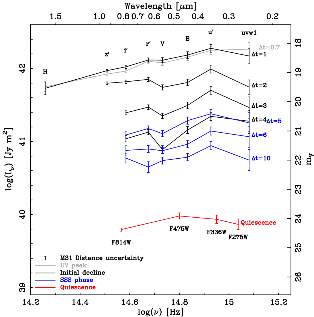
Figure 16. Distance and extinction corrected SED plots showing the evolution of the SED of the 2015 eruption (see key for color identification). Units chosen for consistency with similar plots in Schaefer (2010, see their Figure 71) and DWB14 (see their Figure 4). The central wavelength locations of the Johnson-Cousins, Sloan, HST , and Swift filters are shown to assist the reader. Here the extinction is treated as just the line-of-sight (Galactic) extinction towards M31 ( E_{B-V}^{\text{Galactic}} = 0.1 ; Stark et al. 1992); see the detailed discussion in Darnley et al. (2016c). The error bars include contributions from the photometric and extinction uncertainties, the single black point above the key indicates the systematic uncertainty based on the distance of M31. A V -band apparent magnitude scale (not corrected for extinction) is shown on the right-hand y-axis to aid the reader.
