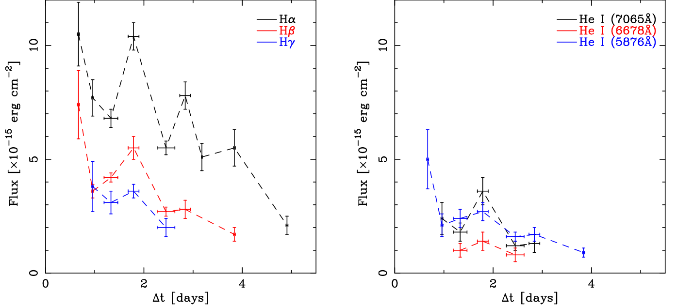
Figure 12. Evolution of the integrated line fluxes of the Balmer (left) and He I (right) lines since the onset of the eruption. Data are from spectra of the 2014, and 2015 eruptions. The dashed-lines connecting the points are to aid the reader only.
