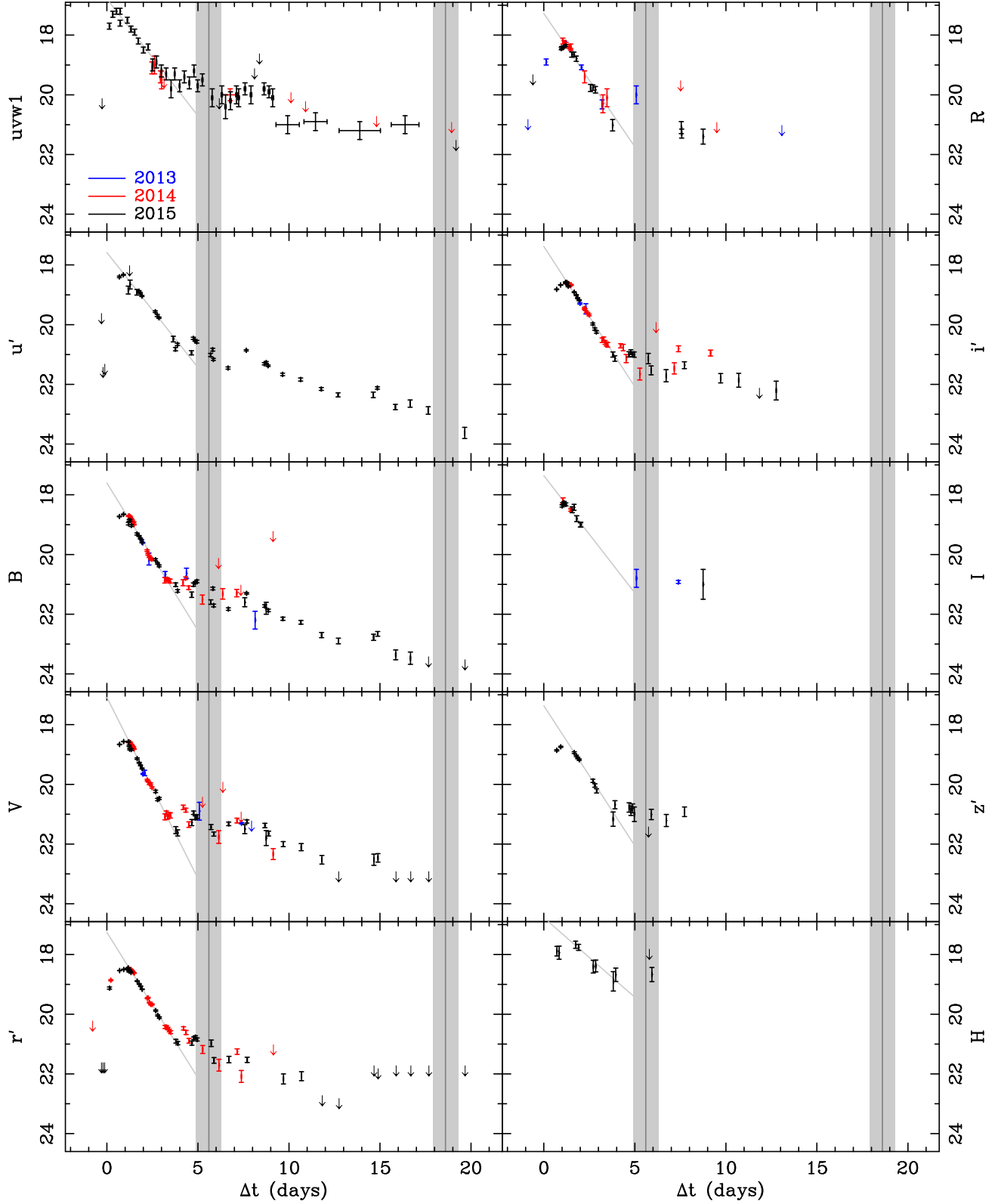
Figure 1. Near-ultraviolet through near-infrared photometry of the 2013–2015 eruptions of M31N 2008-12a. Black points indicate the 2015 eruption, all data taken from Tables D4 and D2, red points indicate data from the 2014 eruption (DHS15; HND15), and blue points the 2013 eruption (DWB14; TBW14). The vertical gray lines indicate the turn-on and turn-off times of the SSS from the 2015 eruption (the shaded areas their associated uncertainties). The gray lines show a linear fit (exponential decay in luminosity) to each light curve between 1 \leq \Delta t \leq 4 days (see Table 4 for the decline times and other characteristics).
