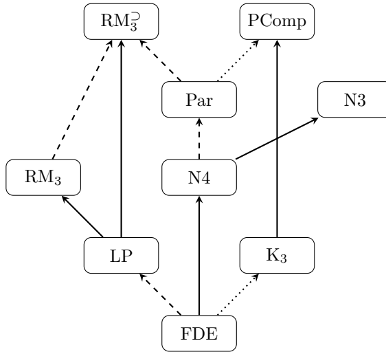
Figure 1. A Hasse-style diagram of the logics in question ordered by inclusion. By dashed lines we indicate that a logic extends another only by rules of inference, by ordinary lines we indicate that a logic extends another also by connectives, by dotted line we indicate that a logic can be formulated as an extension of another only by rules of inference, but we also consider its version obtained by adding the constant falsum.
