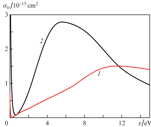
Figure 3. Transport cross sections for electron scattering from argon (1) and xenon (2) atoms.
