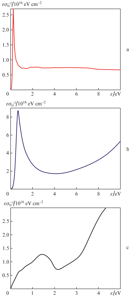
Figure 5. \varepsilon/\sigma_{tr} as a function of electron energy for argon (a), xenon (b), and nitrogen (c).
