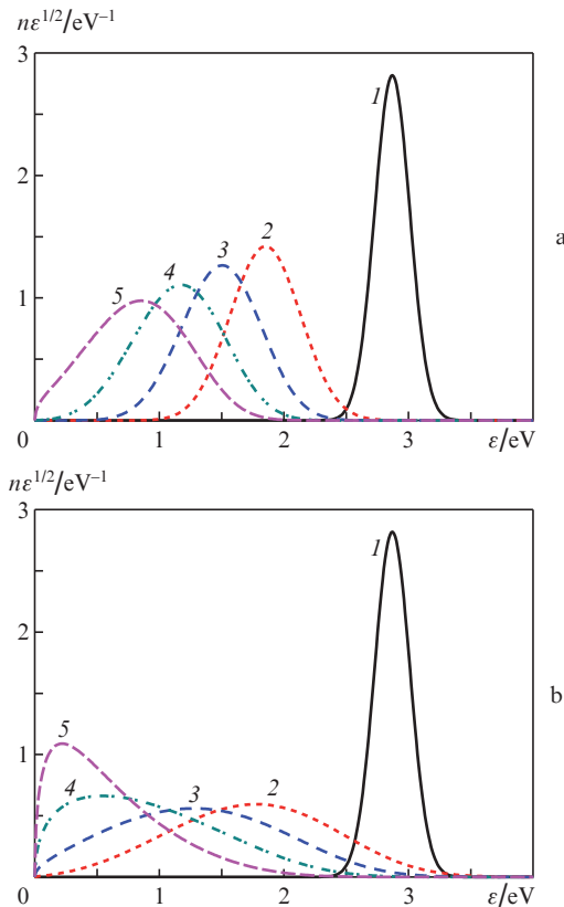
Figure 10. EEDF for xenon at the points in time t = (1) 0 , (2) 25 , (3) 50 , (4) 100 , and (5) 200 \text{ ns} after plasma channel production by \lambda = 248 \text{ nm} radiation. These calculations were carried out with the inclusion of electron–electron collisions for (a) N_e = 10^{12} and (b) 10^{13} \text{ cm}^{-3} .
