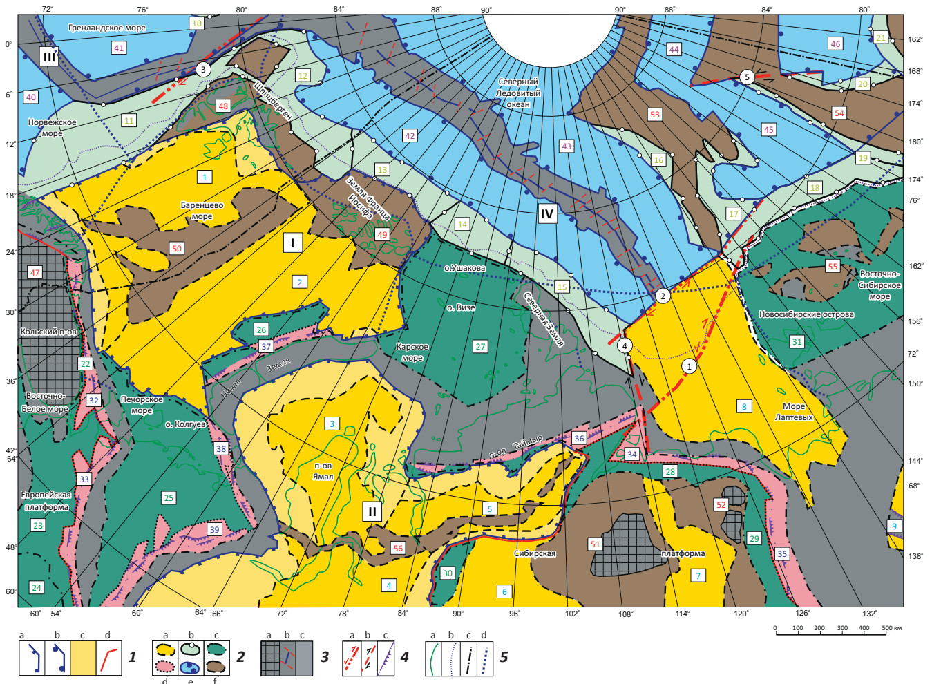
Fig. 1. Largest structures in sedimentary cover of the Western Arctic and neighbouring regions
