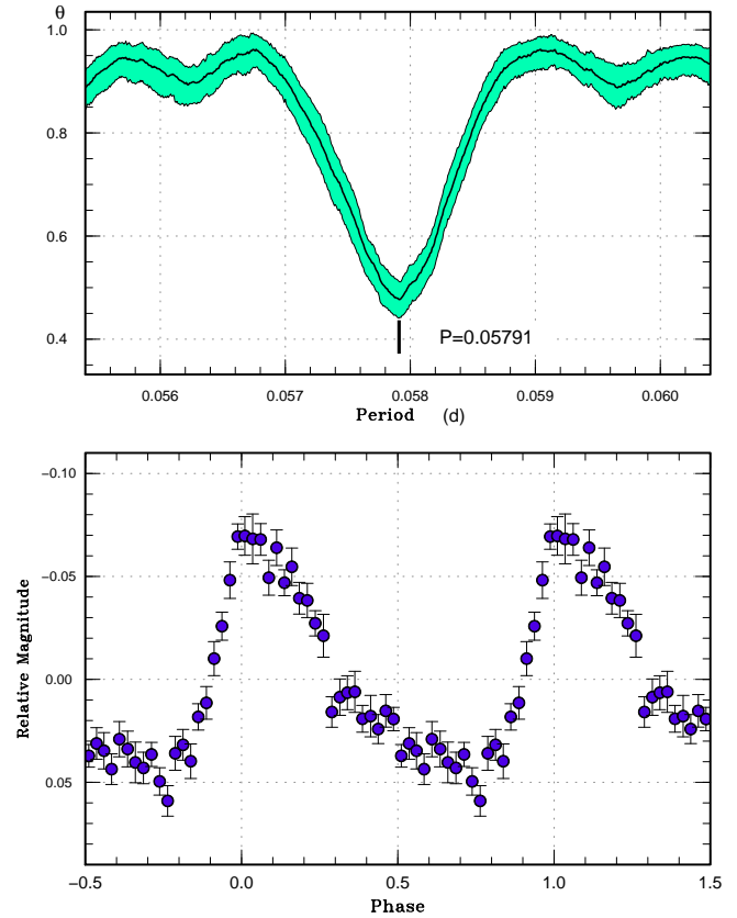
E-figure 71. Ordinary superhumps in ASASSN-17kp (2017). The data before the dip were used. (Upper): PDM analysis. (Lower): Phase-averaged profile.
