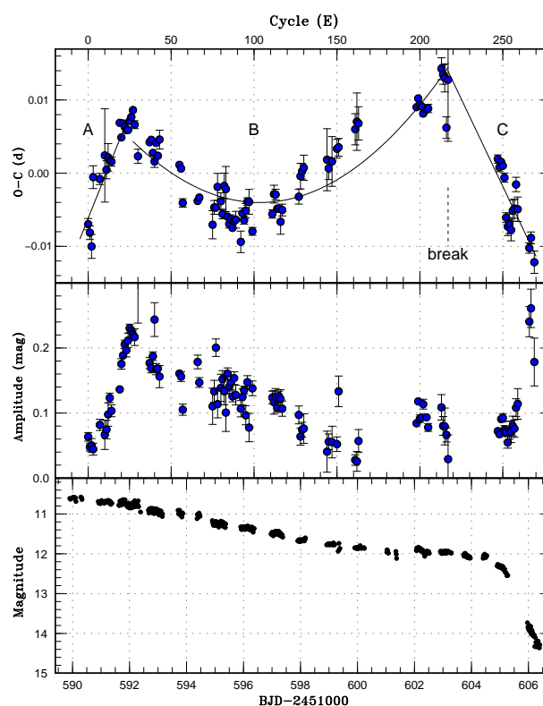
E-figure 1. Representative O - C diagram showing three stages (A–C) of O - C variation. The data were taken from the 2000 superoutburst of SW UMa. (Upper:): O - C diagram. Three distinct stages (A – evolutionary stage with a longer superhump period, B – middle stage, and C – stage after transition to a shorter period) and the location of the period break between stages B and C are shown. (Middle): Amplitude of superhumps. During stage A, the amplitude of the superhumps grew. (Lower:): Light curve. (Reproduction of figure 1 in Kato and Osaki 2013)
