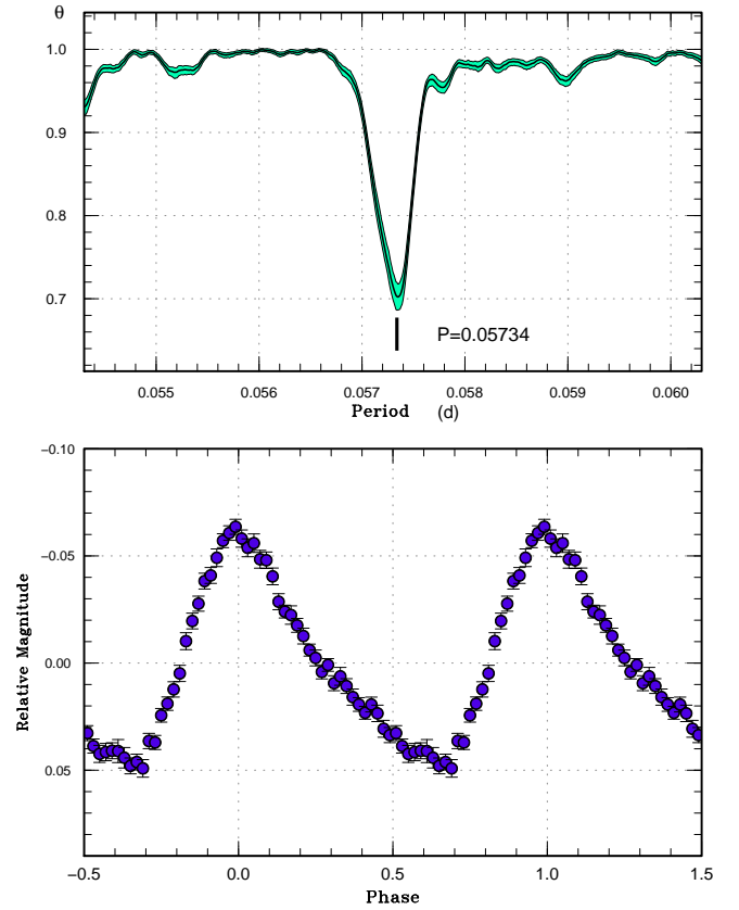
E-figure 95. Ordinary superhumps in PNV J202053 (2017). (Upper): PDM analysis. (Lower): Phase-averaged profile.
