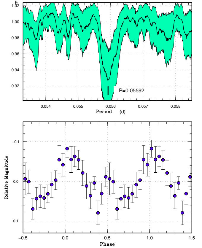
E-figure 63. Superhumps in ASASSN-17iw (2017). (Upper): PDM analysis. (Lower): Phase-averaged profile.
