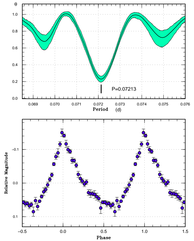
E-figure 34. Superhumps in ASASSN-17eq (2017). (Upper): PDM analysis. (Lower): Phase-averaged profile.
