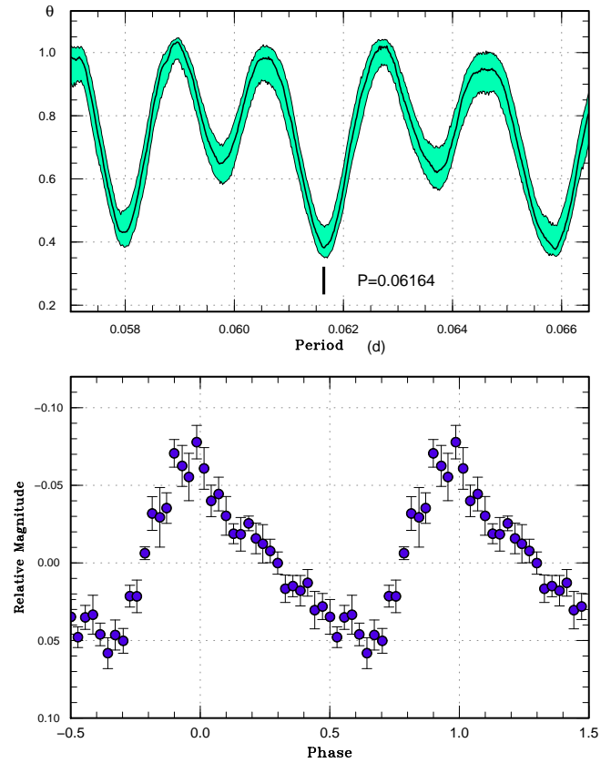
E-figure 98. Superhumps in SDSS J204817 (2009). (Upper): PDM analysis. (Lower): Phase-averaged profile.
