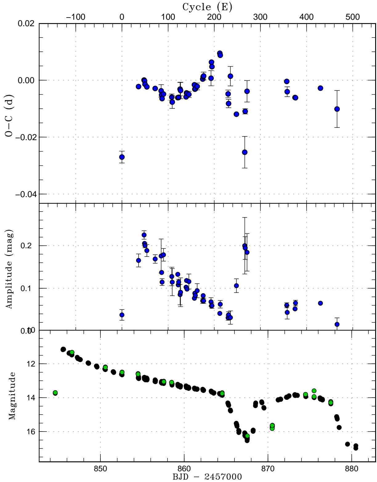
E-figure 33. O - C diagram of superhumps in ASASSN-17el (2017). (Upper:) O - C diagram. We used a period of 0.055132 d for calculating the O - C residuals. (Middle:) Amplitudes of superhumps. (Lower:) Light curve. The black filled circles are our CCD data binned to 0.018 d. The green filled circles are ASAS-SN V measurements. There were also our CCD observations at the same locations of a dip in ASAS-SN measurements at BJD 2457870.5.
