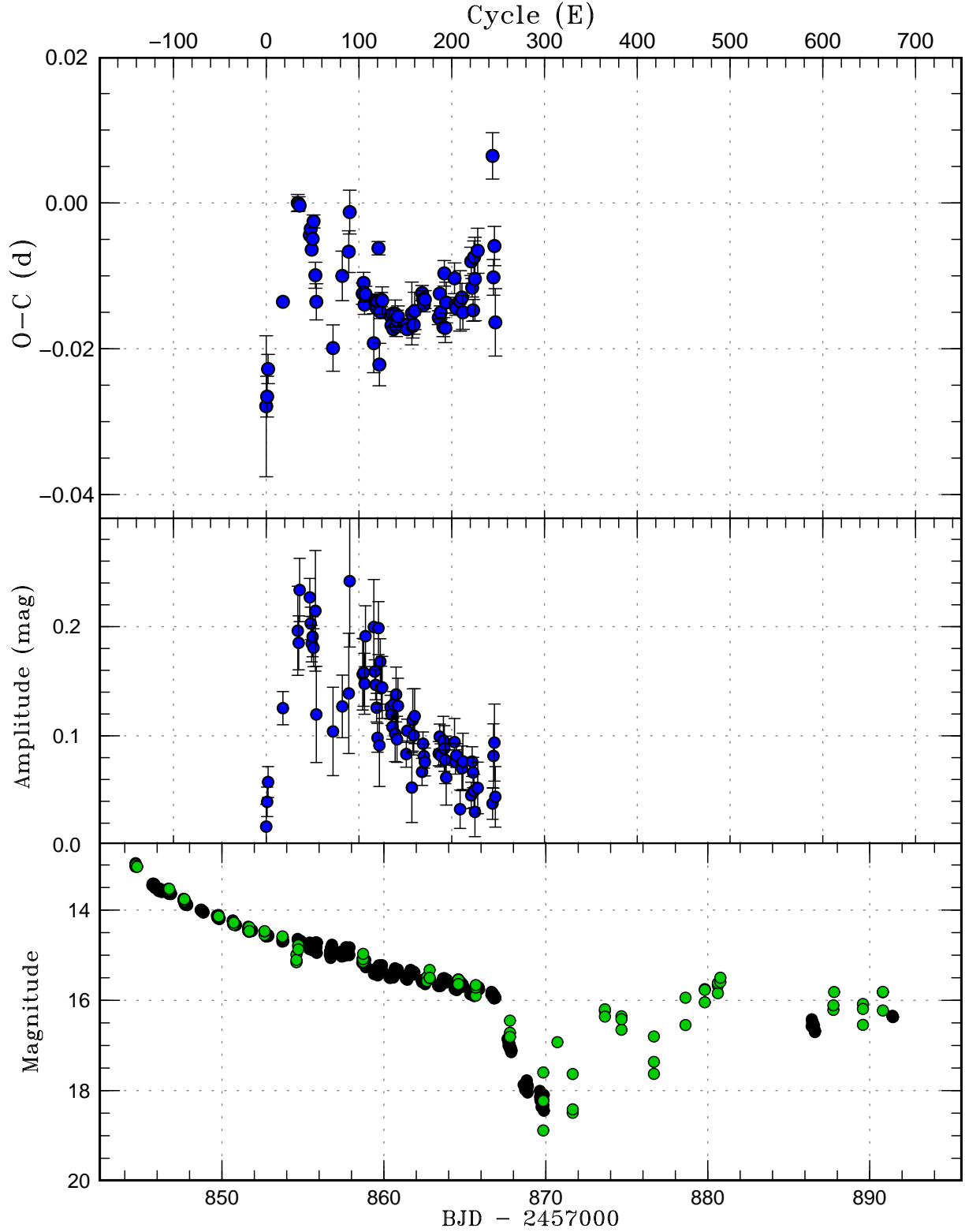
E-figure 30. O - C diagram of superhumps in ASASSN-17ei (2017). (Upper:) O - C diagram. We used a period of 0.05728 d for calculating the O - C residuals. (Middle:) Amplitudes of superhumps. (Lower:) Light curve. The black filled circles are our CCD data binned to 0.019 d. The green filled circles are ASAS-SN V measurements. A constant flux corresponding to V=16.64 has been subtracted to best match time-series CCD observations.
