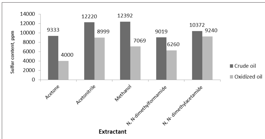
Figure 1 – Dependence of residual sulfur content on the nature of the extractant. (Conditions: S: \text{H}_2\text{O}_2 (50%): \text{HCOOH} = 1: 10: 6 (mol.), 20 °C, 6 hours)
