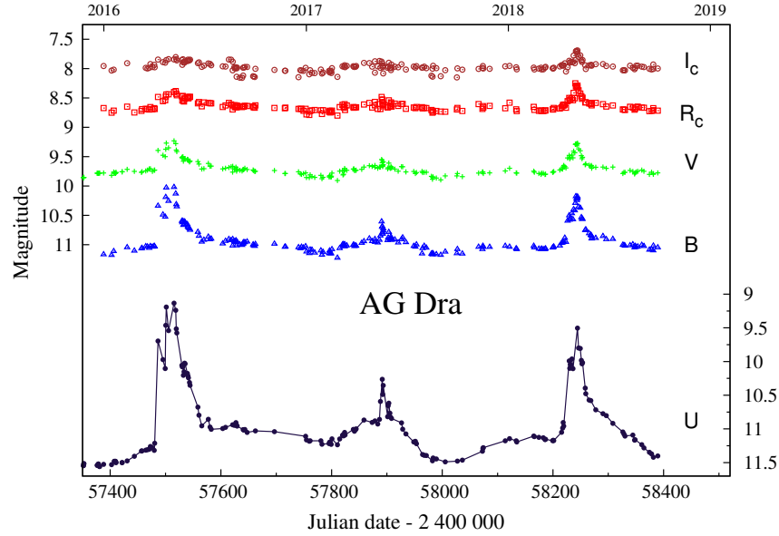
Figure 19. Recent three outbursts of AG Dra. Note the multi-peaked structure for the 2016 one.
