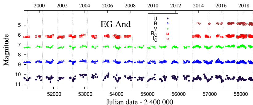
Figure 1. UBVRcIc LCs of EG And. Vertical lines represent times of the inferior spectroscopic conjunction of the giant according to the ephemeris of Kenyon & Garcia (2016), JD_{\text{sp.conj.}} = 2450208.108(\pm 0.672) + (482.5 \pm 1.3) \times E . New observations are displayed with those of Skopal et al. (2012).
