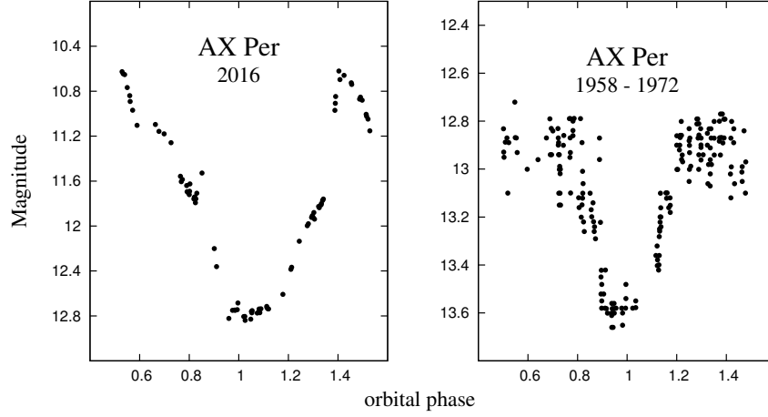
Figure 31. A comparison between the shape of the 2016 eclipse during the current active phase and eclipses during the 1958-1972 quiescent period (data are from Myalkovskij, 1977).
