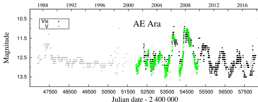
Figure 6. The LC of AE Ara consisting of visual estimates from the AAVSO database (grey dots), our data (black) and V magnitudes from ASAS database (green).
