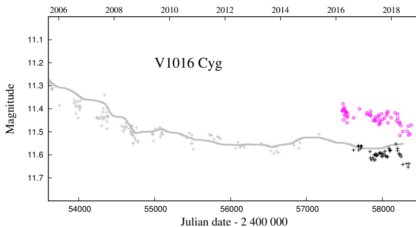
Figure 14. The V LC of V1016 Cyg using different instruments. Gray crosses are data from Arkhipova et al. (2008, 2015, 2016a,b), black crosses are from the private station (M.V.) and G1 pavilion, while the magenta circles are data obtained in the G2 pavilion (see Sect. 2). The grey line represents smoothed LC of visual estimates from the AAVSO database shifted by +0.33 mag.
