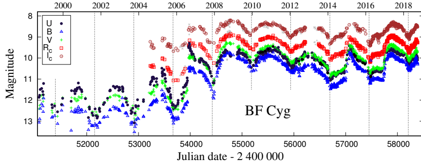
Figure 8. As in Fig. 1, but for BF Cyg. Vertical lines represent times for conjunctions with the giant in front according to the ephemeris of Fekel et al. (2001), JD_{\text{sp.conj.}} = 2\,451\,395.2(\pm 5.6) + (757.2 \pm 3.9) \times E . Our new observations are displayed with the data published by Skopal et al. (2007, 2012), Yudin et al. (2005) and, for a comparison, data from the AAVSO database (grey points).
