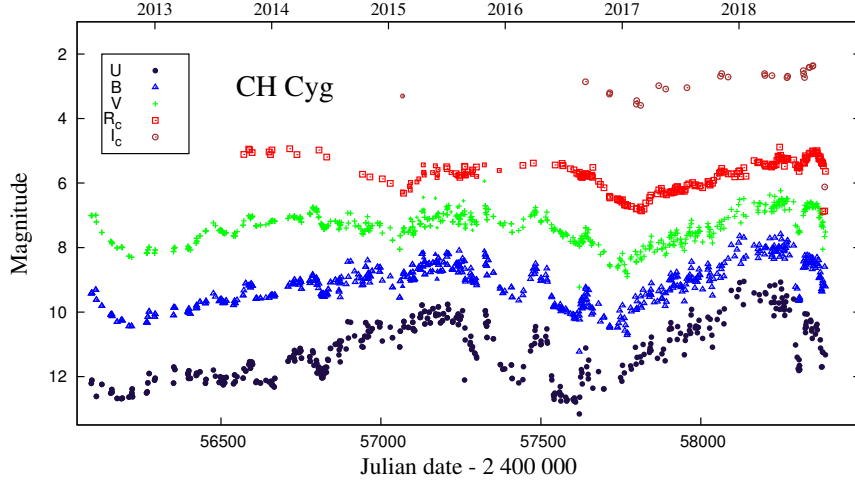
Figure 10. Detail of Fig. 9 from 2012.4. The U and B LCs were shifted by 3 and 0.7 mag, respectively, for better visualization.
