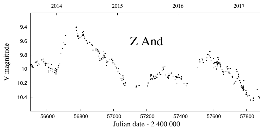
Figure 5. The V LC of Z And from the AAVSO database (grey points) and our measurements (black points). Observations suggest the presence of a 58-d periodic variability.
