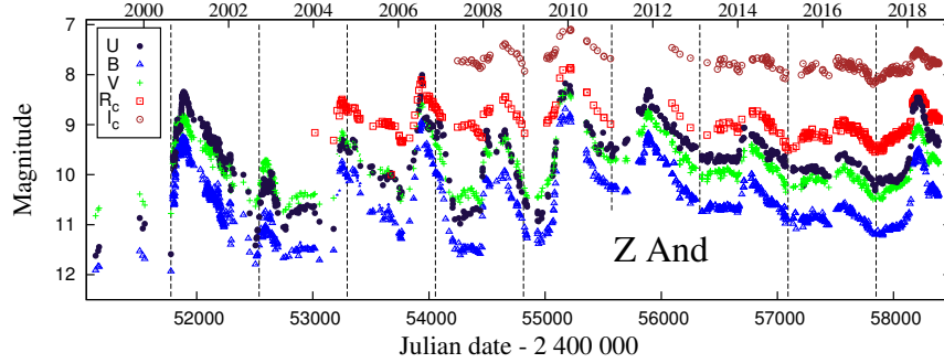
Figure 4. As in Fig. 1, but for Z And. Times of the inferior conjunctions of the giant (vertical lines) are according to the ephemeris of Fekel et al. (2000a), JD_{\text{sp.conj.}} = 2\,450\,260.2(\pm 5.4) + (759.0 \pm 1.9) \times E . Data from Skopal et al. (2007, 2012) are supplemented by our data from 2011.9.
