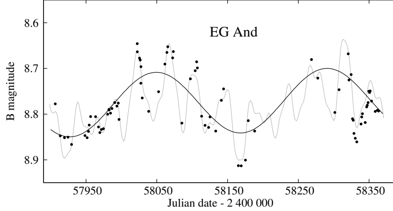
Figure 3. A part of the B LC of EG And, where a light variation with peaks separated by several tens of days is clearly recognized. The grey line represents a model including periods: 241 (half of the P_{\text{orb}} – black line), 39, 46, and 28 days (see text).
