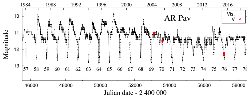
Figure 23. The visual LC of AR Pav made by two observers (AJ and RS). Our new observations (see Sect. 2) are displayed with the V data from the AAVSO database (Rolf Carstens) and those published by Skopal et al. (2004, 2007).
