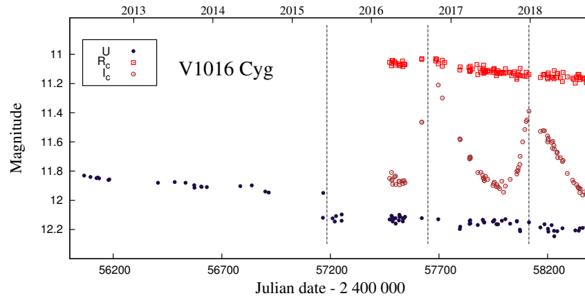
Figure 15. A sudden decrease in the U brightness of V1016 Cyg (around 2015.4) could be connected with pulsations of the Mira variable. The vertical lines correspond to times of the maximum light in the I_C filter for the period of 465 days. First six points after the decrease are adapted from Fig. 1 of Arkhipova et al. (2016a). Their uncertainties are <0.01 mag and \pm 10 days in the scale of magnitudes and JD, respectively.
