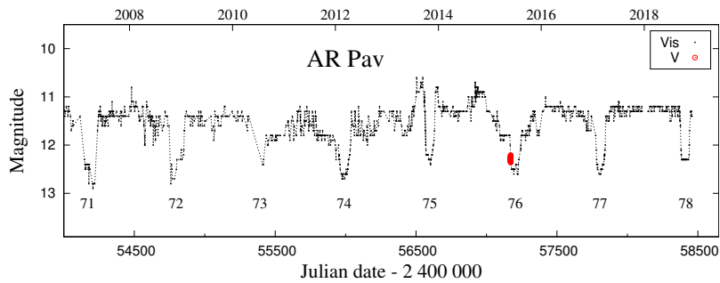
Figure 24. The recent low stage of AR Pav between the epoch 71 and 78.
