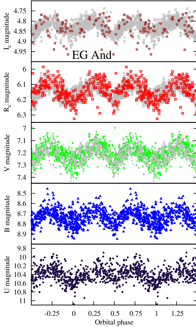
Figure 2. Phase diagrams of our UBVR_CI_C magnitudes for EG And. Compared are VRI data of Percy et al. (2001) shifted by an appropriate constant (in grey). The large scatter of the data is caused by several types of variabilities (see text).
