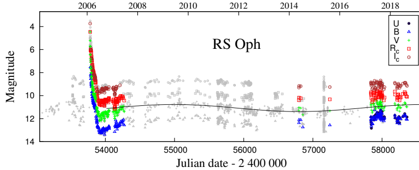
Figure 21. As in Fig. 1, but for RS Oph. Our new observations are displayed with the data of Hachisu et al. (2008) (2006 outburst) and from the AAVSO database (grey). The solid line represents a sine function with amplitude \Delta V \sim 0.3 mag and a period of \sim 9.4 years.
