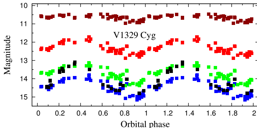
Figure 17. Phase diagram of our UBVR_{CI} magnitudes of V1329 Cyg. We used the ephemeris for the pre-outburst minima (eclipses) as derived by Schild & Schmid (1997), JD_{\text{Min}} = 2\,427\,687(\pm 20) + (958.0 \pm 1.8) \times E . Denotation of points as in Fig. 1.
