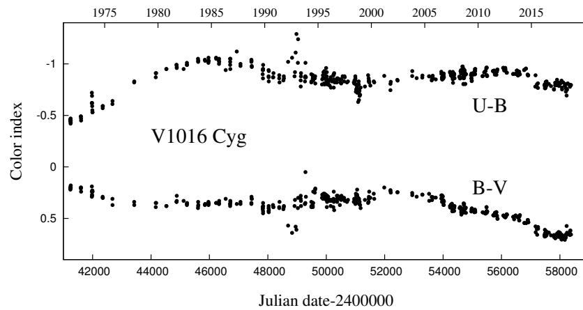
Figure 16. Evolution of colour indices of V1016 Cyg. Data sources as in Fig. 13.
