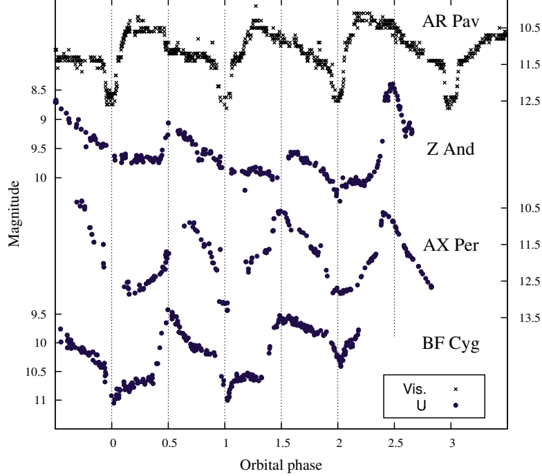
Figure 30. Comparison of the recent AX Per LC with those of other active symbiotic stars. The light maximum and minimum usually appear around \varphi \sim 0.5 and \sim 0 , respectively, while the LC of AR Pav shows maxima around \varphi \sim 0.25 .
