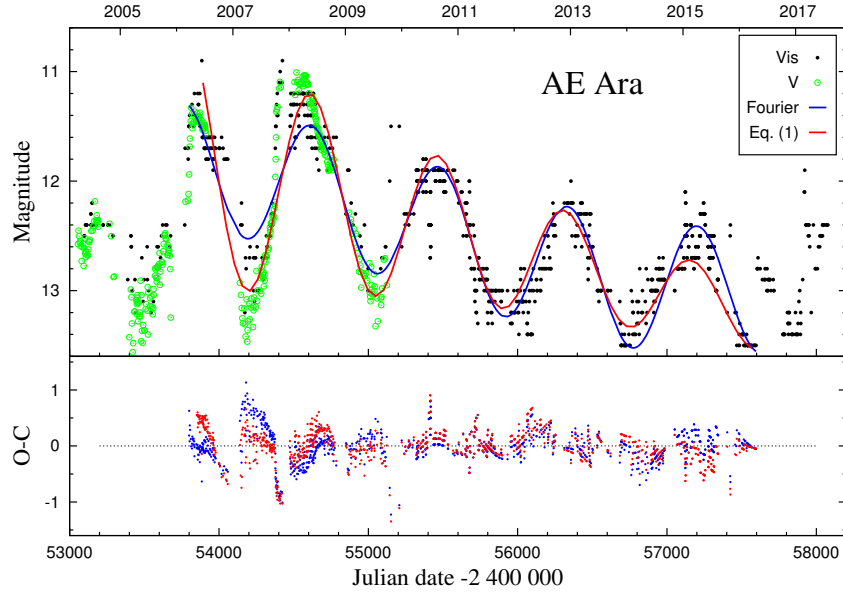
Figure 7. Top: Our fits to the V /visual LC of AE Ara during its transition from the active to quiescent phase (2006.2 – 2016.6). The corresponding orbital period is larger than that determined from the quiescent LC (see text). Bottom: O - C residuals between the fit from Fourier analysis (blue points), Eq. (1) (red points) and the data.
