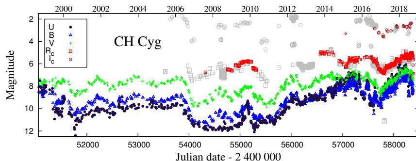
Figure 9. As in Fig. 1, but for CH Cyg. New data (from 2011.9) are supplemented with those published by Skopal et al. (2007, 2012) and the AAVSO R_C magnitudes (grey points).
