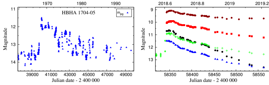
Figure 33. Left: Historical LC of HBHA 1704-05 obtained from the Moscow’s photographic plates archive. Right: Our UBVR_{CI} LCs measured from the maximum of the outburst, on August 12, 2018. Compared are the ASASSN V magnitudes prior to the outburst. Denotation of points as in Fig. 1.
