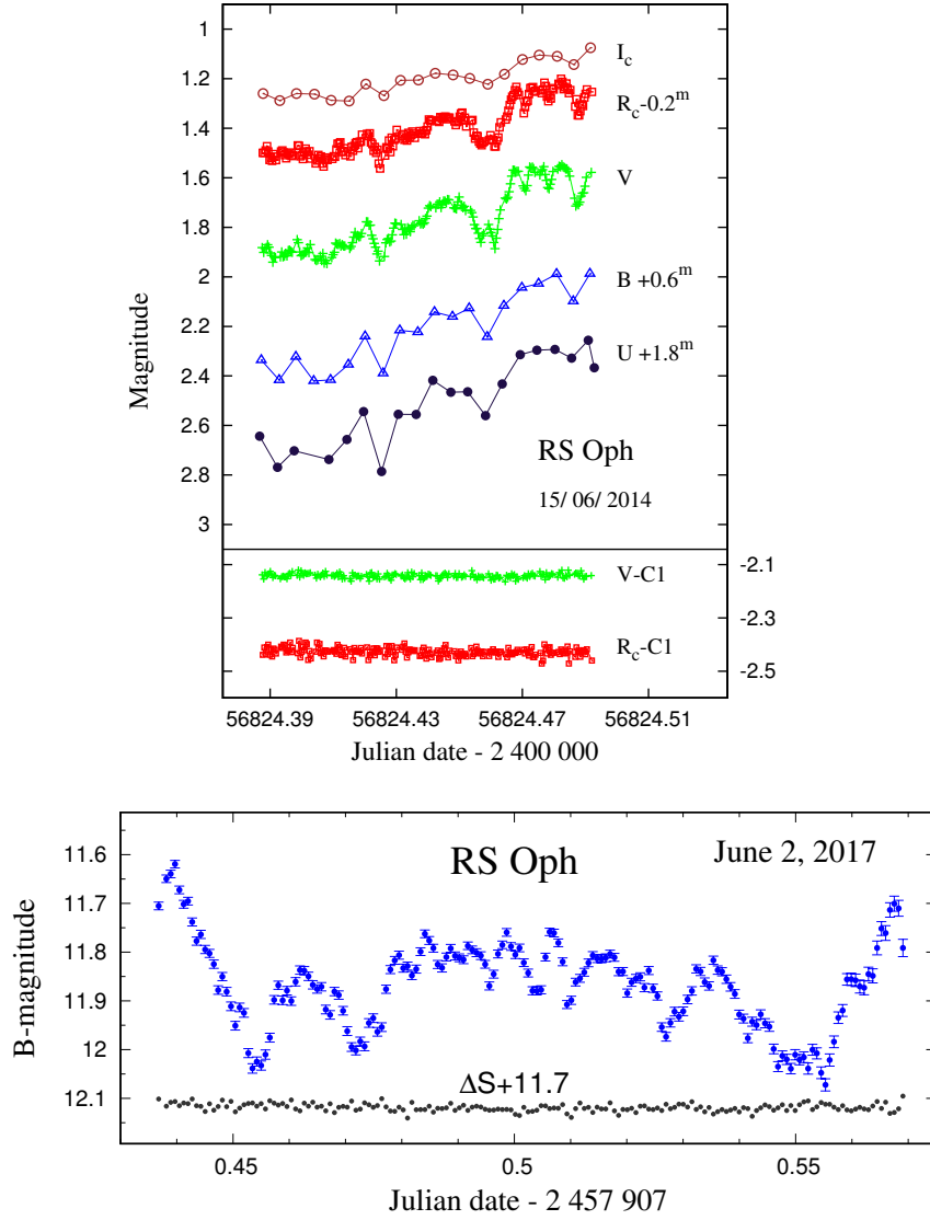
Figure 22. Examples of rapid photometric variability of RS Oph. Top panel shows variations in UBVR_CI_C filters obtained in G2 pavilion (point (ii) of Sect. 2), while the bottom panel shows high-cadence observations in B acquired at the private station (point (iii) of Sect. 2). Here, we used the star UCAC4-417-071413, ( V=9.307 mag, B-V=1.236 ) as the comparison and UCAC4-416-072918 as the check star. \Delta S denotes their difference in B .
