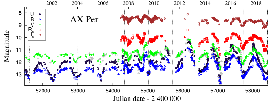
Figure 28. As in Fig. 1, but for AX Per. Vertical lines represent the timing of eclipses, JD_{\text{Ecl.}} = 2447551.26(\pm 0.3) + (680.83 \pm 0.11) \times E (Skopal et al., 2011). New data are complemented with those of Skopal et al. (2011, 2012) and V from AAVSO (grey).
