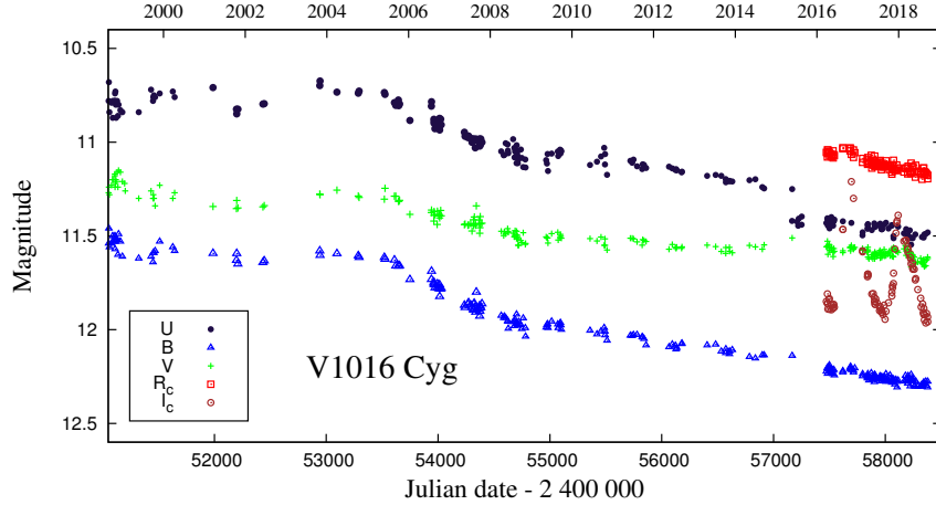
Figure 13. As in Fig. 1, but for V1016 Cyg. Here, our new observations are displayed with those published by Parimucha et al. (2000) and Arkhipova et al. (2008, 2016a,b).
