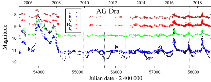
Figure 18. As in Fig. 1, but for AG Dra. Vertical lines represent inferior conjunctions of the giant according to the ephemeris of Fekel et al. (2000a), JD_{\text{sp.conj.}} = 2\,450\,775.3(\pm 4.1) + (548.65 \pm 0.97) \times E . Our new observations are displayed with the data published by Skopal et al. (2012) and Munari et al. (2009b).
