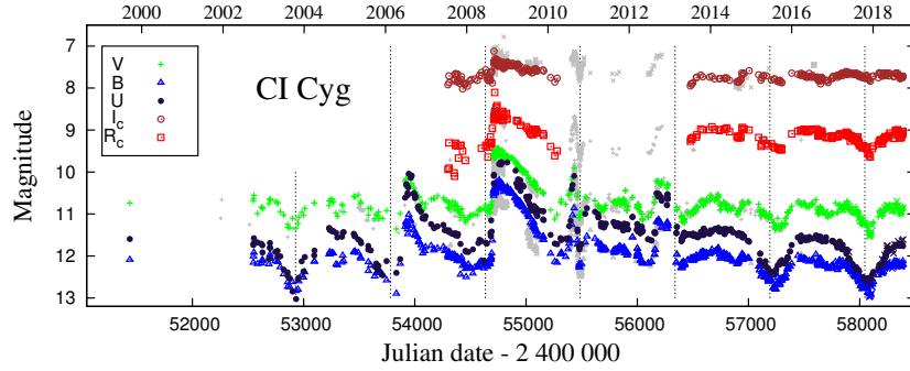
Figure 11. As in Fig. 1, but for CI Cyg. The timing of eclipses is given by the ephemeris of Skopal et al. (2012), JD_{\text{Ecl.}} = 2441838.8(\pm 1.3) + (852.98 \pm 0.15) \times E . Our observations are displayed with those of Skopal et al. (2007, 2012), Siviero et al. (2009) and from AAVSO (grey).
