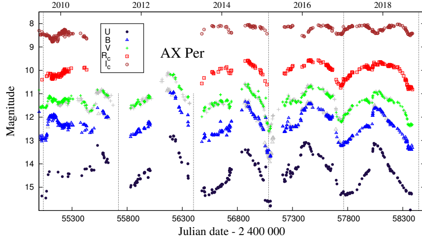
Figure 29. The recent evolution of the AX Per LCs covering its current active stage. The U LC is shifted by +2.5 mag for better visualization.
