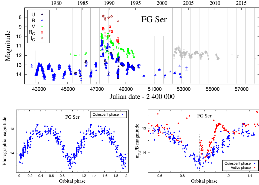
Figure 32. Top: As in Fig. 1, but for FG Ser. The vertical lines represent times of minima according to Eq. (3). The figure displays our photographic magnitudes from archives, data published by Kurochkin (1993) (shifted by -0.2 mag) and photographic and photoelectric data of Munari et al. (1992, 1995) (other colours). Compared are visual estimates from AAVSO (grey). Bottom: phase diagram of m_{pg} magnitudes during quiescent phase (left; JD < 2\,447\,000 ) and its comparison with B measurements from the 1988-94 active phase (right).
