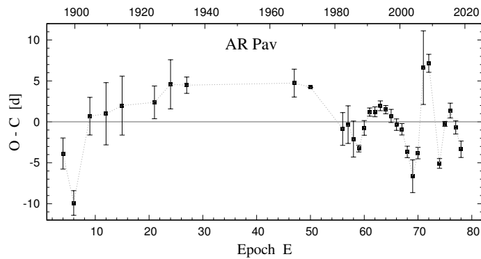
Figure 25. O-C diagram for the linear ephemeris (2) determined by timing of eclipses (Table 2) in the historical LC of AR Pav.
