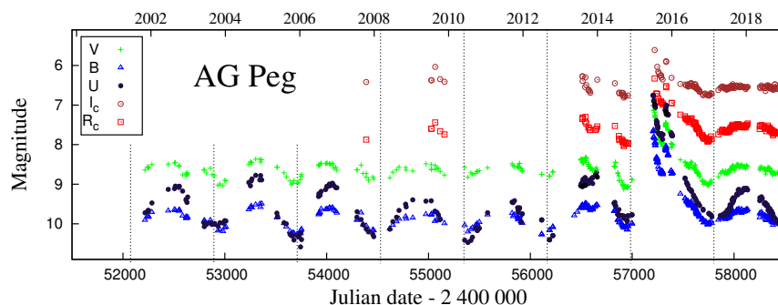
Figure 26. As in Fig. 1, but for AG Peg. Data to 2011.9 were published by Skopal et al. (2012). Vertical lines represent inferior conjunctions of the giant according to ephemeris of Fekel et al. (2000b), JD_{sp.conj.} = 2\,447\,165.3(\pm 48) + (818.2 \pm 1.6) \times E .
