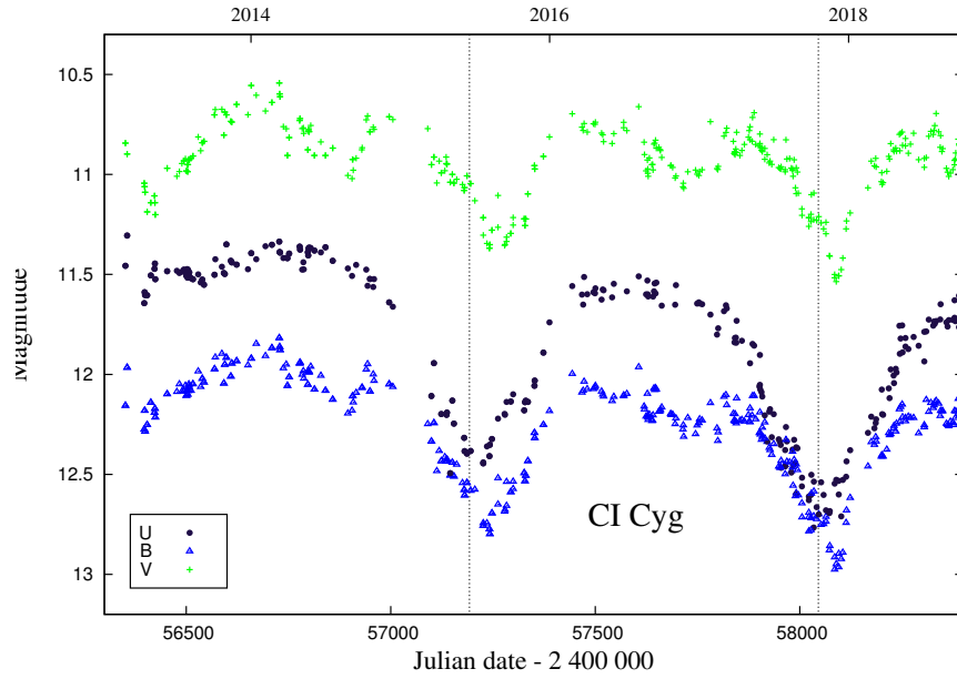
Figure 12. During the last two orbital cycles, wave-like orbitally-related variation developed in the LC of CI Cyg – a signature of quiescent phases of symbiotic stars (see Sect. 1). Secondary minima around \varphi \sim 0.6 are indicated in B and V . In the V LC, a variation with a period of \sim 73 days can be found. Vertical lines as in Fig. 11.
