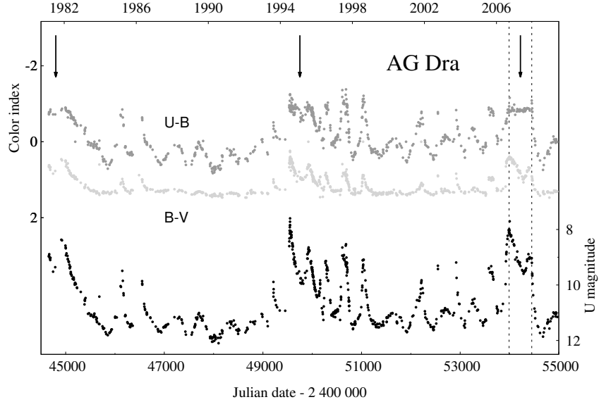
Figure 20. The (U - B) colour shows a plateau during the cool 2006-07 outburst of AG Dra. Vertical lines bounds its duration. Also during previous major outbursts (1981-82, 1994-95) the index was relatively stable (arrows).
