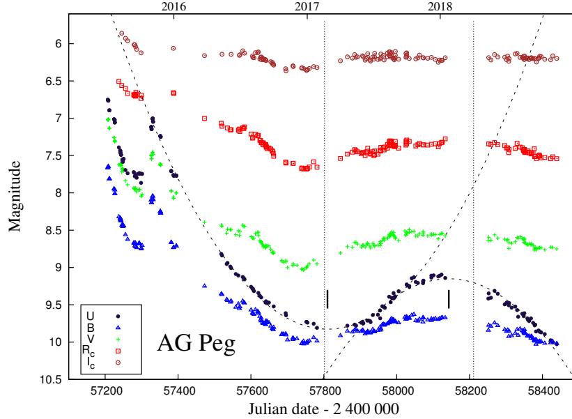
Figure 27. Multicolour LCs after the 2015 outburst demonstrating transition of AG Peg to quiescent phase. Dashed curves are quadratic functions, vertical lines represents orbital phase 0 (JD 2 457 801.9) and 0.5 (JD 2 458 211.0) and short vertical bars mark corresponding minimum and maximum in U .
