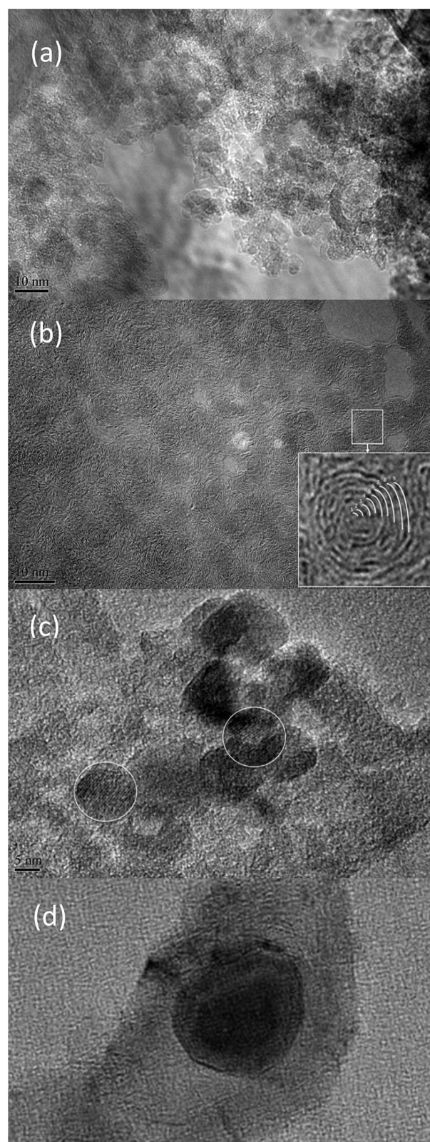
Fig. 5 TEM images of porous graphitic carbon composites. (a) Amorphous carbon, (b) carbon onions resulting from the thermal annealing of detonation nanodiamond (DND) under \text{N}_2 at 1250 °C, (c) DND remains intact within the porous graphitic carbon composite following pyrolysis up to 900 °C, (d) DND showing surface graphitisation following pyrolysis up to 900 °C.
