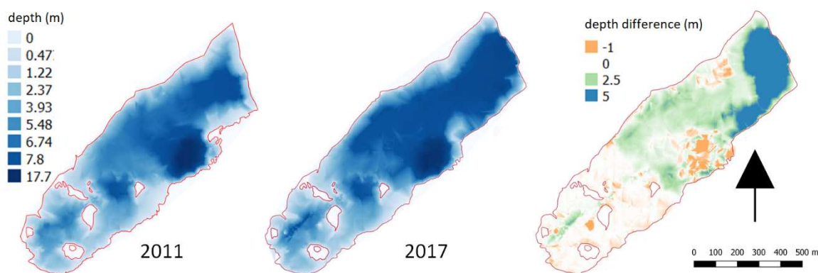
Figure 2 Changes in lake bathymetry.
