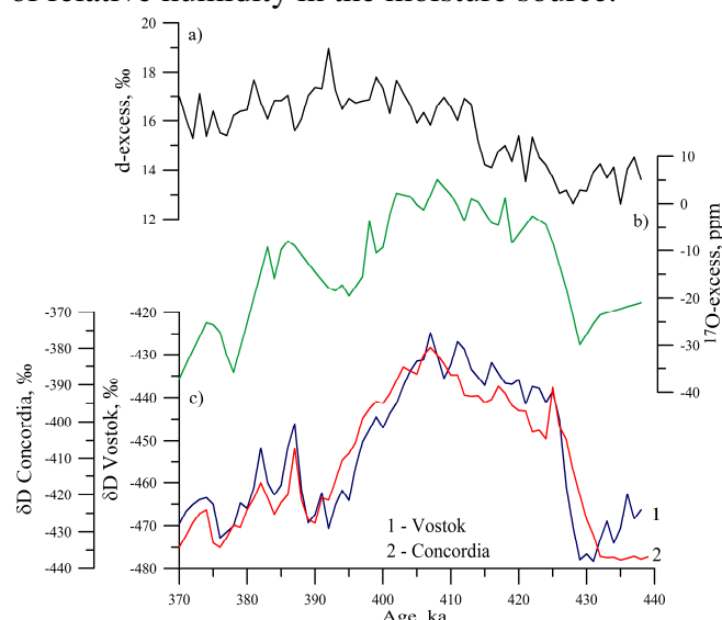
Figure 1 Time series of isotopic characteristics based on the Vostok ice core measurements over the period of 370–440 ka BP: a – d-excess; b – ^{17}O -excess; c – \delta D : 1 – the Vostok ice core; 2 – the Concordia ice core [1].
